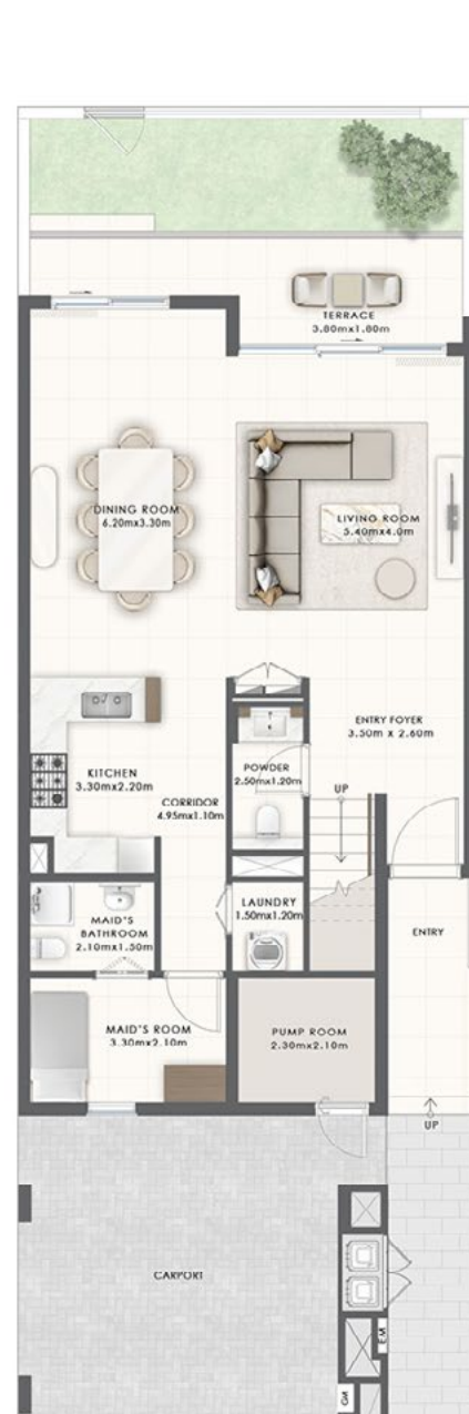
GROUND FLOOR
